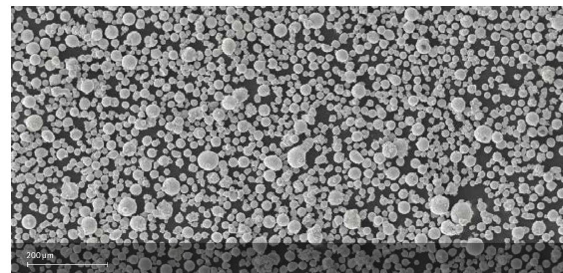
SEM picture of EOS ToolSteel 1.2709 powder.
