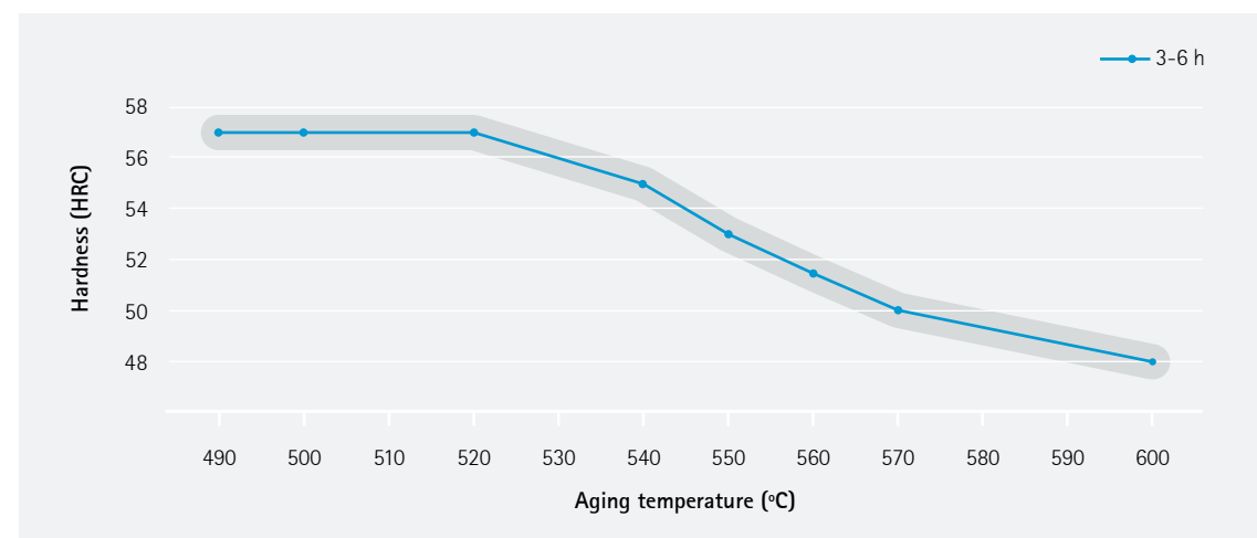
If lower hardness and improved toughness is required, aging temperature can be increased according to figure above.
